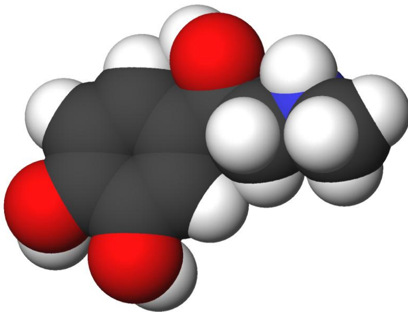
Figure 3. 3-dimensional structure of Adrenaline
